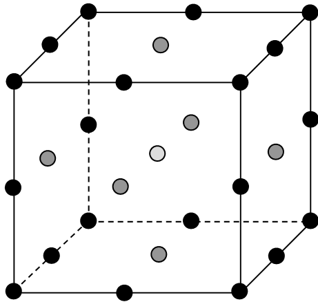
Fig. 27-node hexahedral element
