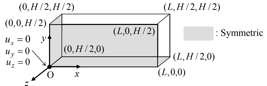
(b) Boundary conditions
